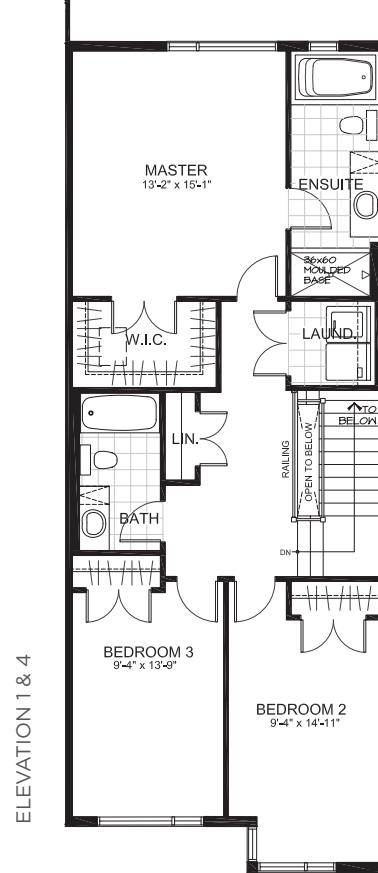
SECOND FLOOR ALT 3 BEDROOMS
