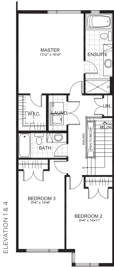
SECOND FLOOR 3 BEDROOMS
